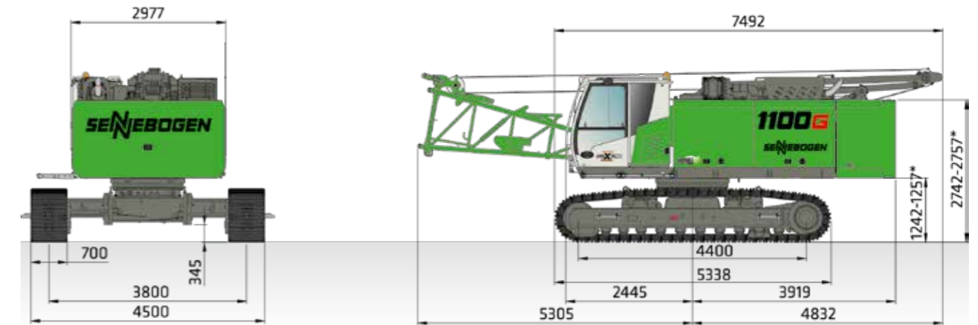
1100 G with 18 t counterweight, telescopic undercarriage T41/380, lower boom section, 2 x 12 t winch, approx. 48,400 kg
