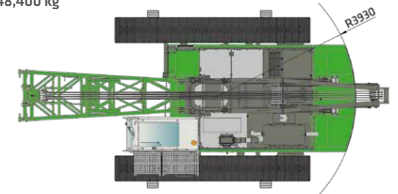
1100 G with 18 t counterweight, telescopic undercarriage T41/380, lower boom section, 2 x 12 t winch, approx. 48,400 kg
