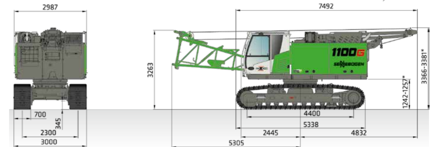
1100 G without counterweight, lower boom section, 2 x 12 t winch, approx. 30,400 kg
